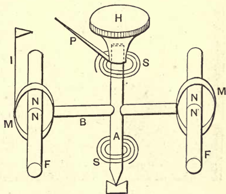
Fig. 76.—Principle of Fleming and Gimmingham's Dynamometer Voltmeter
